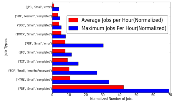
Figure 9. Normalized Average and maximum job counts per hour for the top 10 job types (for 1 week).
