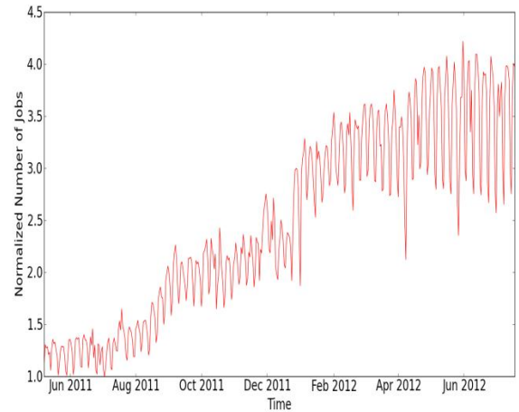
Figure 4. Normalized number of jobs per day.
