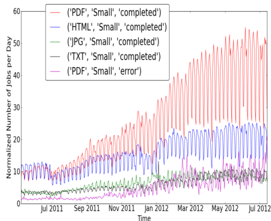
a) Top 5 Job Types
