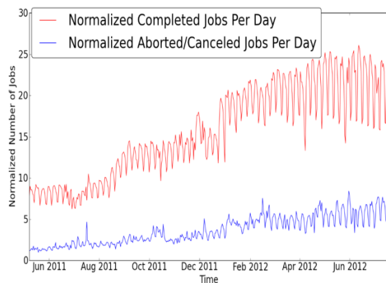
Figure 5. Normalized number of completed and error/aborted/canceled jobs per day.
