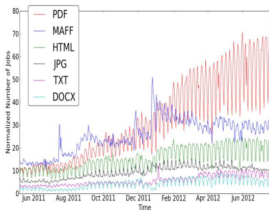
Figure 6. Normalized number of jobs per format per day.
