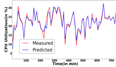
Figure 12. Predicted vs measured CPU utilization for a Linux worker node.
