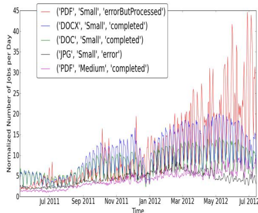
b) Next 5 Job Types
