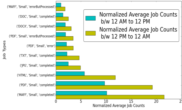
Figure 11. Normalized Average number of jobs for top 10 job types during a different times of day.
