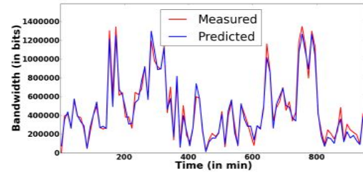
Figure 13. Predicted vs measured bandwidth for a Linux worker node.
