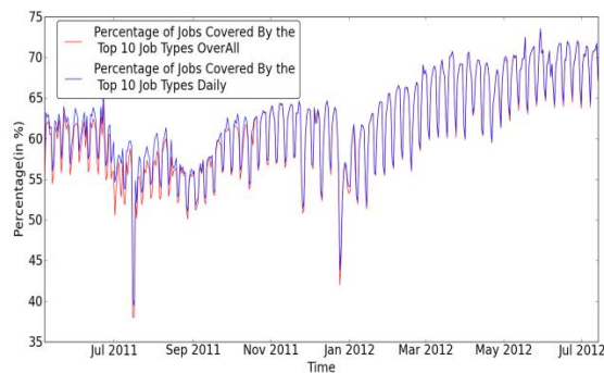
c) Percentage of jobs covered by top 10 job types (10 top jobs overall and 10 top jobs daily)
