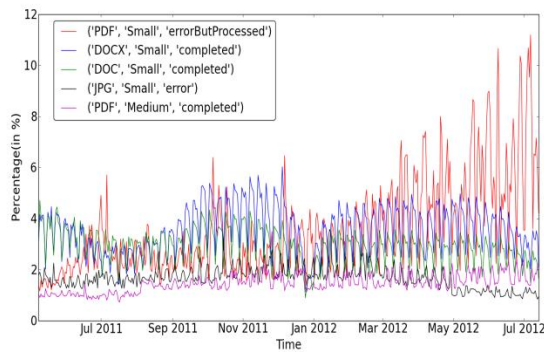
b) Percentage of jobs covered by next 5 job types per day
