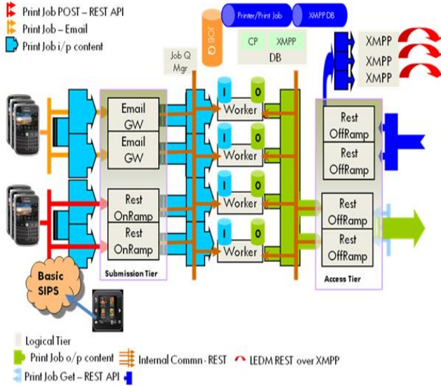
Figure 1. High-level view of HP ePrint System.
