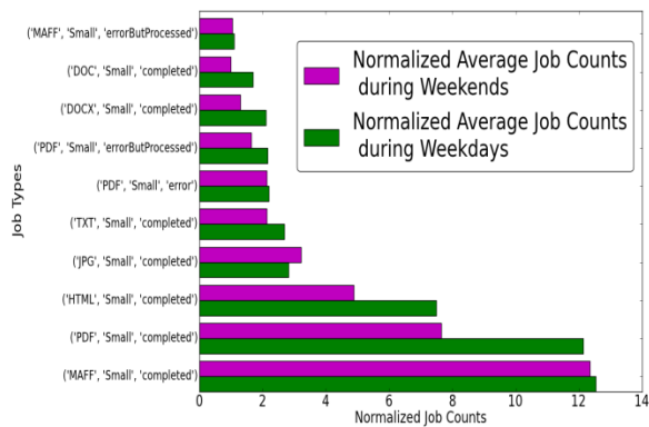
Figure 10. Normalized Average number of jobs for top 10 job types during weekdays and weekends.
