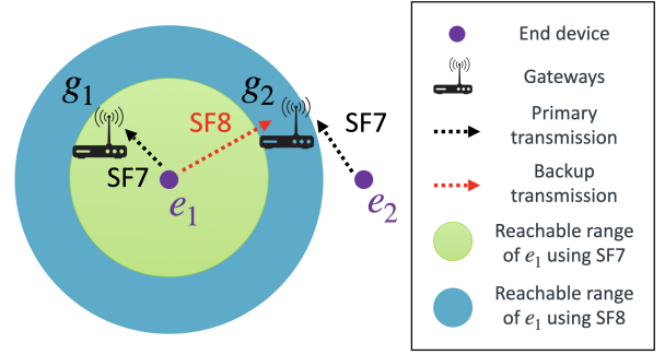
Fig. 1: An example of 2-gateway connectivity setup on end device e_1 .
