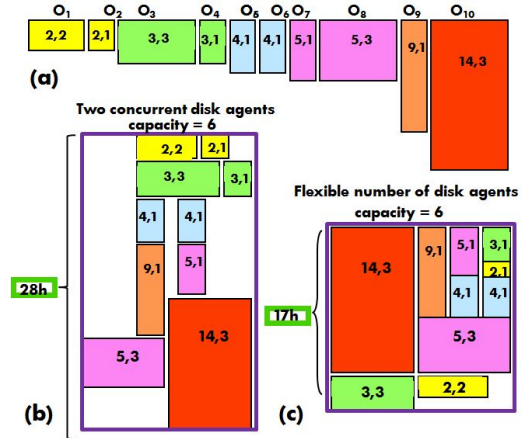
Fig. 2. Motivating example.
