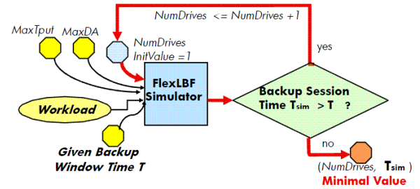
Fig. 5. Simulation routine: determining the minimal number of drives.
